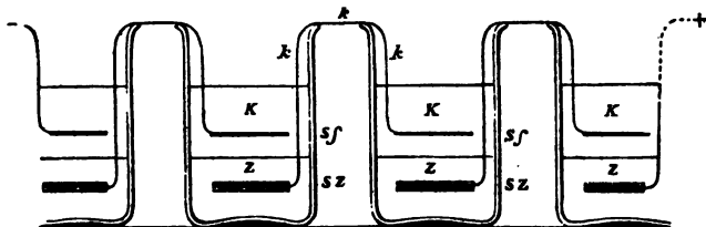
EXPERIMENT ILLUSTRATING THE ARGUMENT OF BERZELIUS FOR THE 'CONTACT' THEORY OF THE ORIGIN OF THE GALVANIC CURRENT
